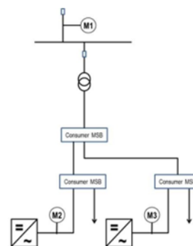
Fig. 9.1: Location of Energy Meters
